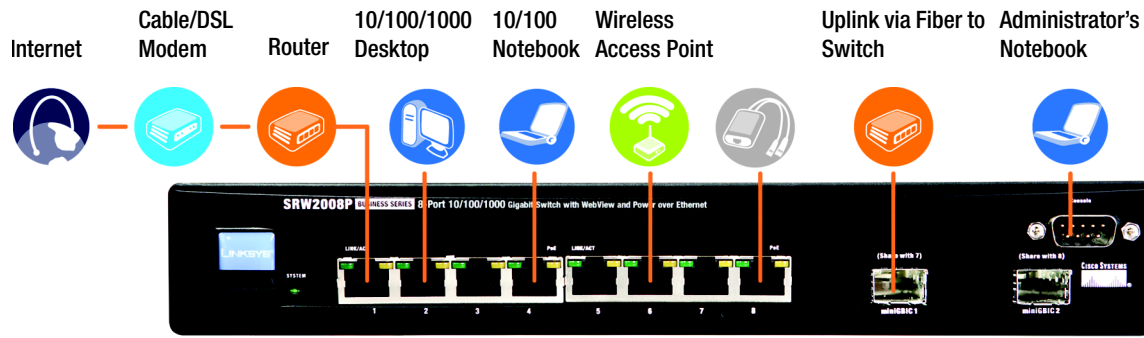
Figure 3-1: Typical Network Configuration for the SRW2008P
